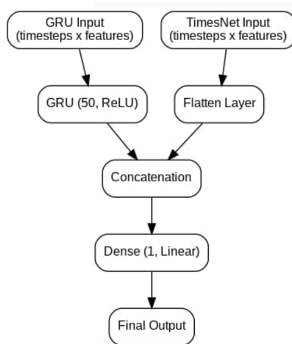
Figure 19: Workflow of GRU+TimesNet model
