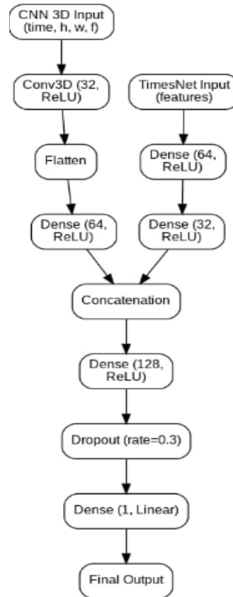
Figure 18: Workflow of CNN 3D+TimesNet model
