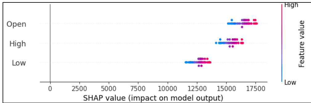
Figure 30: SHAP summary plot for determining feature importance
