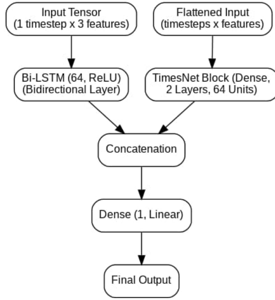
Figure 20: Workflow of TimesNet+Bi LSTM model
