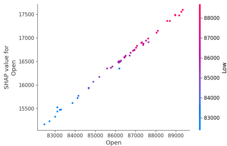
Figure 31: SHAP Dependence plot to determine feature importance
